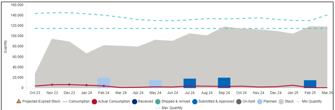
Figure 106 Supply Planning Graph - Primary Axis (Plan by Quantity)
