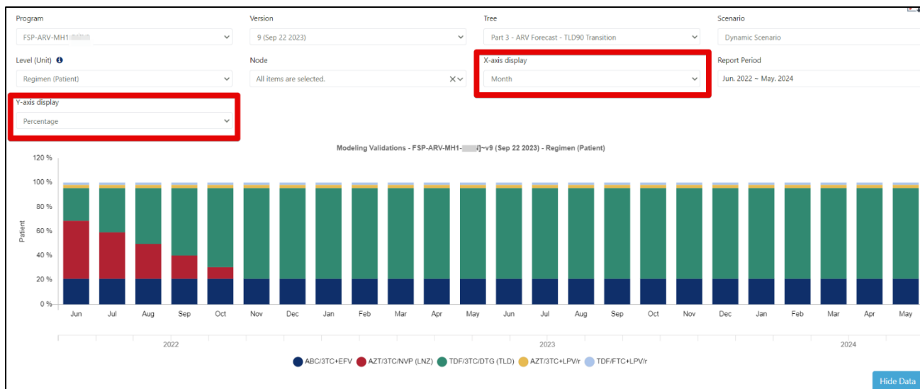
Figure 178: Modeling Validation Screen (by percentage and month)
