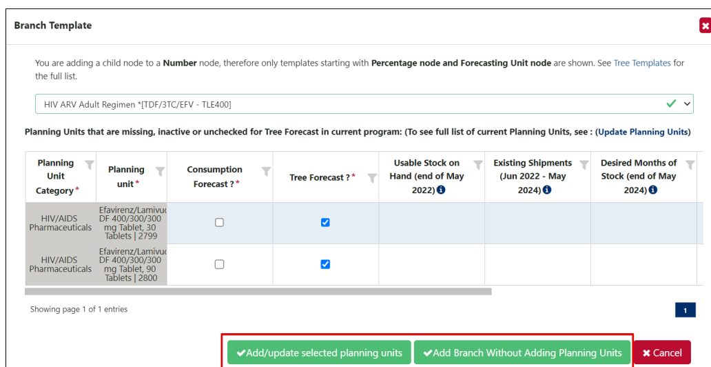
Figure 184: Adding PUs from a Branch Template to a Program
