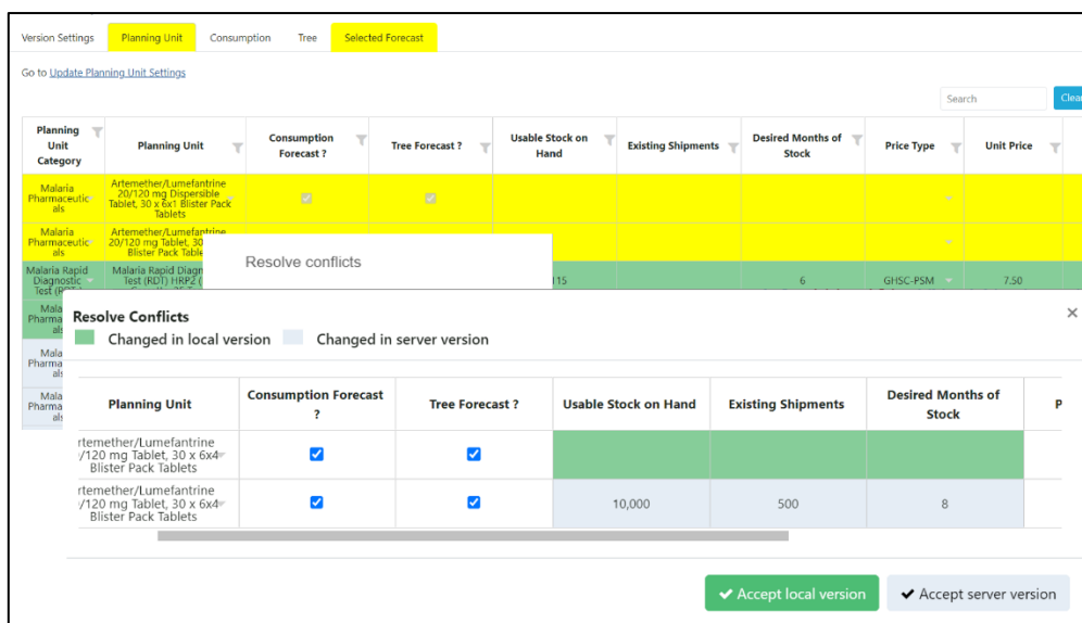
Figure 58 Resolving Conflict while uploading forecast
