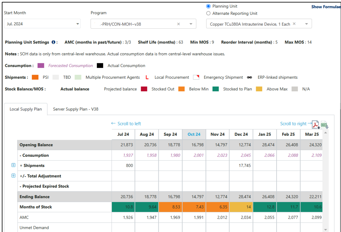
Figure 99: Supply Planning Screen – Plan by MOS
