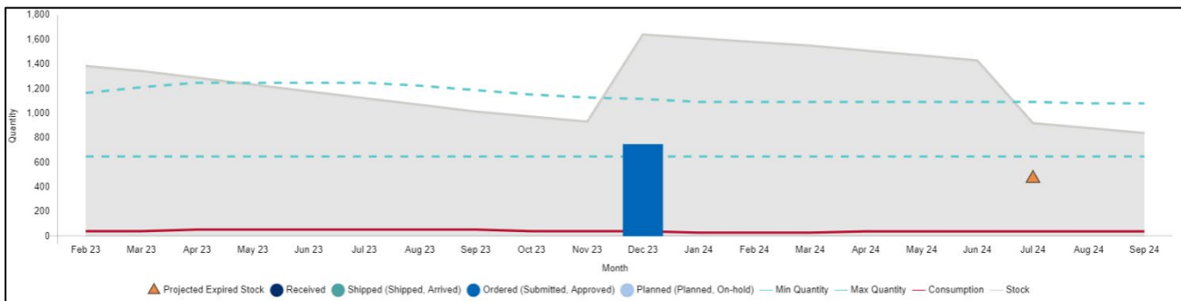
Figure 128: Supply Plan does not follow min/max quantity parameter example
