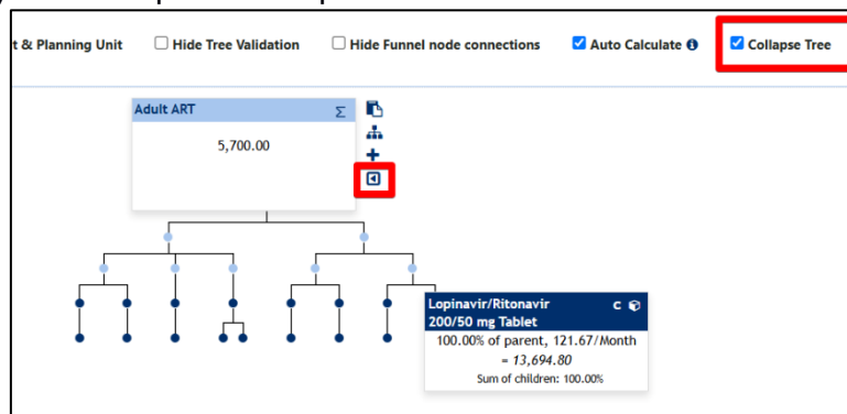
Figure 170: Example of a Collapsed Forecasting Tree
