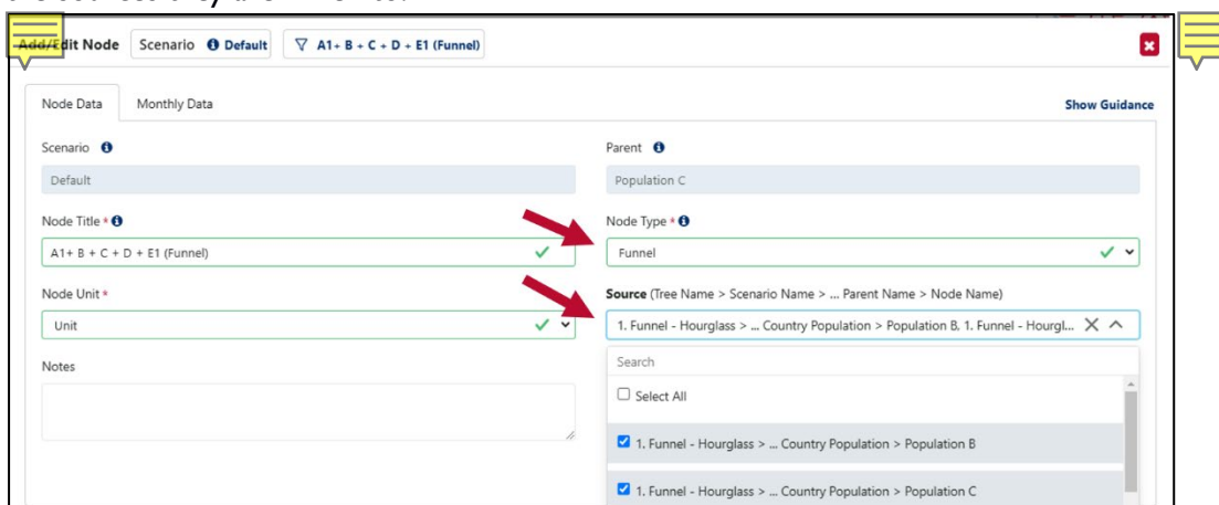
Figure 176 Adding funnel nodes
