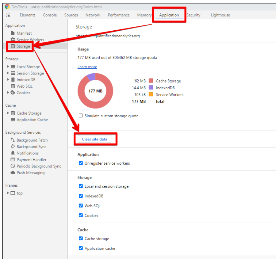
Figure 17: Clear Site Data
