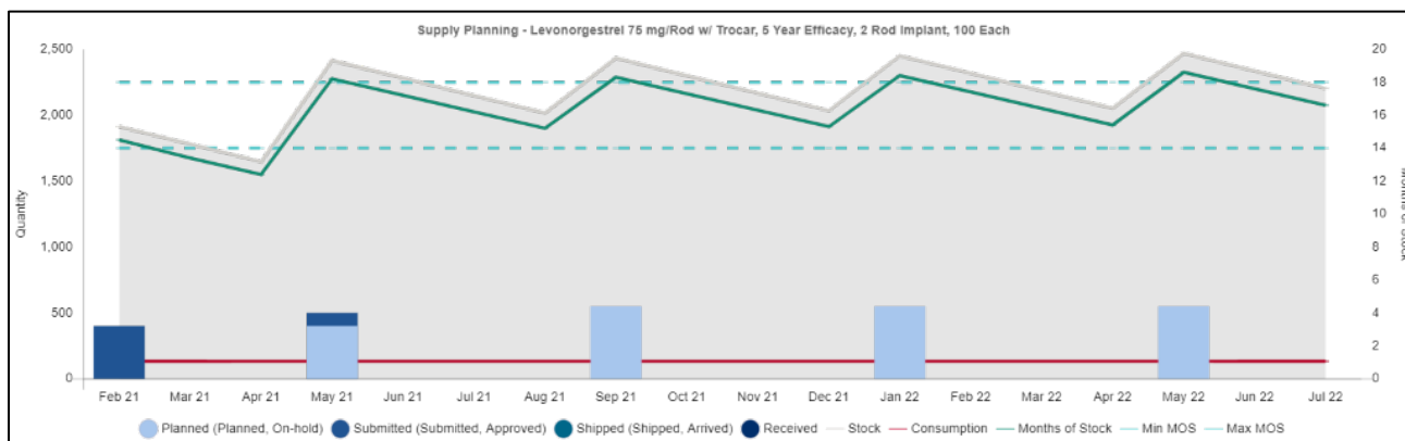
Figure 127: Supply Plan does not follow min/max MOS parameter example
